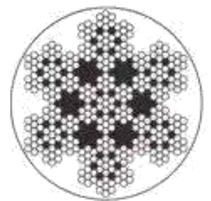
7X7X7
