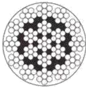
19X7
