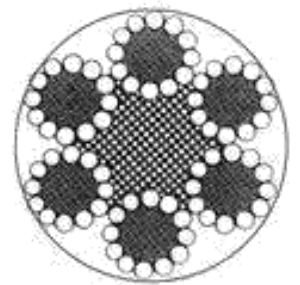
6x12+7FC
