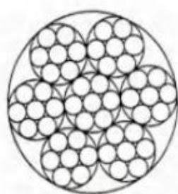
6X7+IWS
